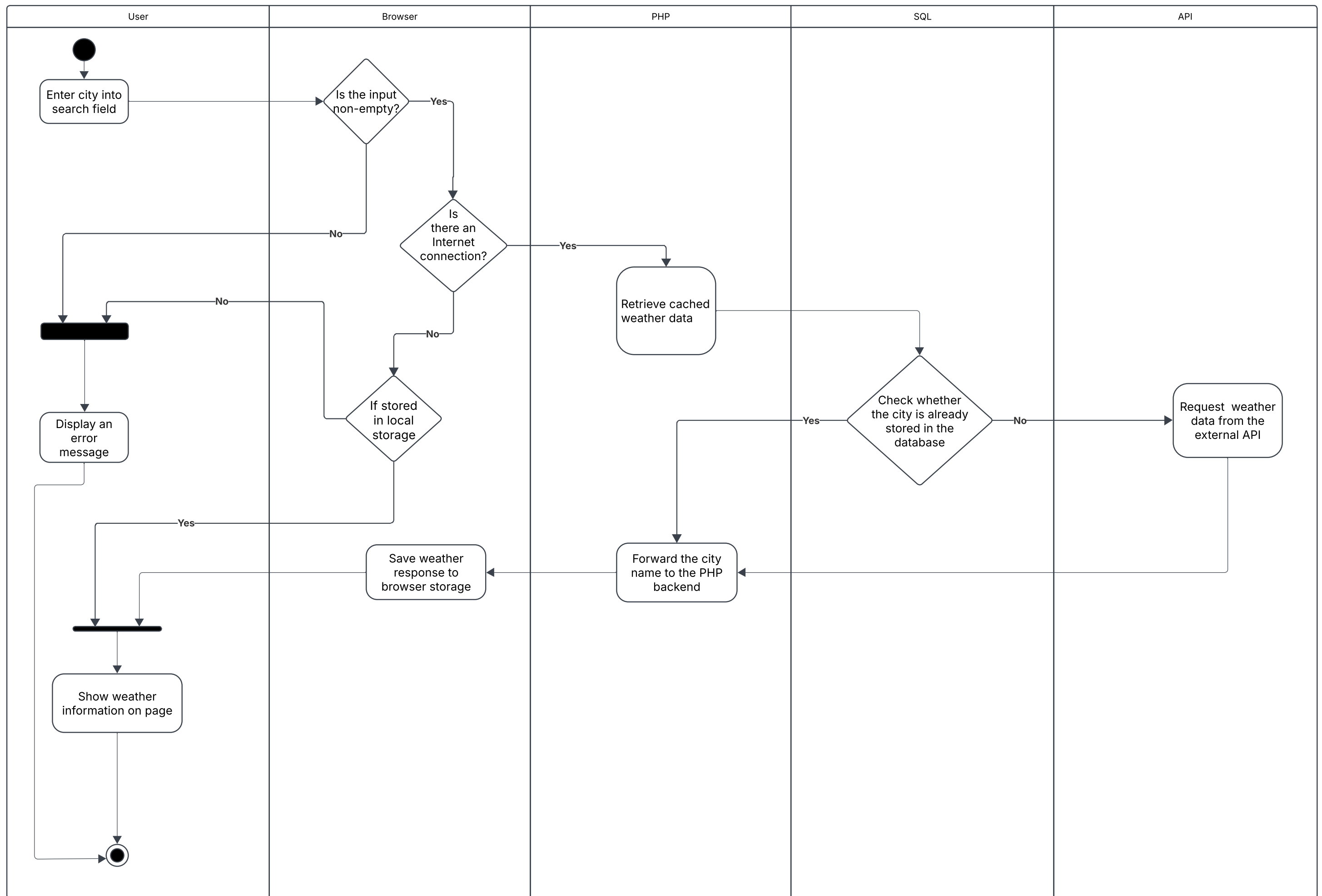
Weather App activity diagram
